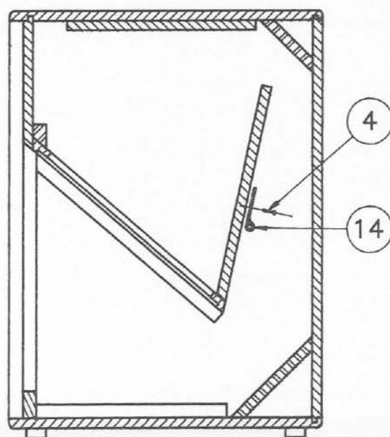
SIDE SECTION
